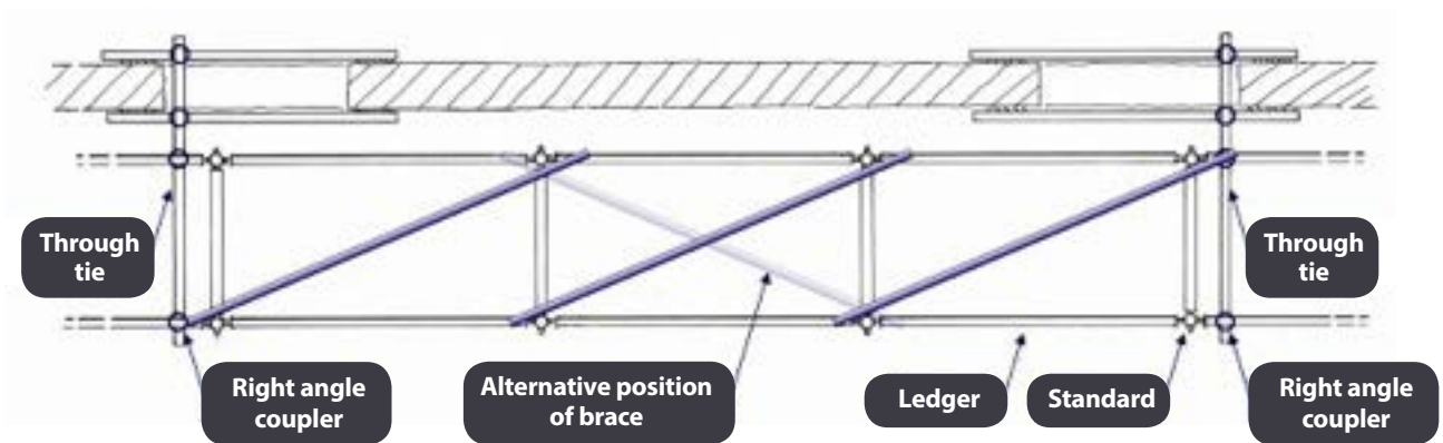
Figure 14: Example of Plan Bracing
